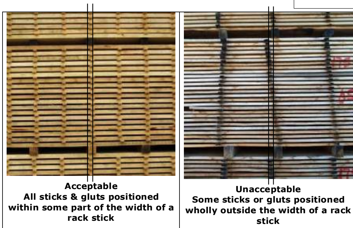
Figure 11.04. Rack stick, glut and bearer alignment
