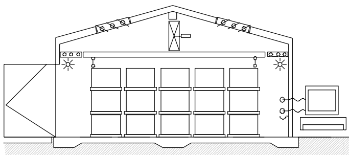
Figure 9.01. Generic layout of conventional predryer
